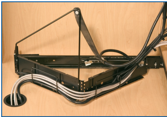
Cable Management - side view
